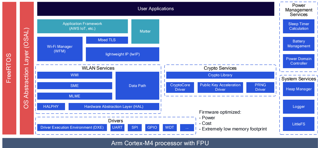
Figure 10: QCC730 Module Development Kit SDK Software Architecture
