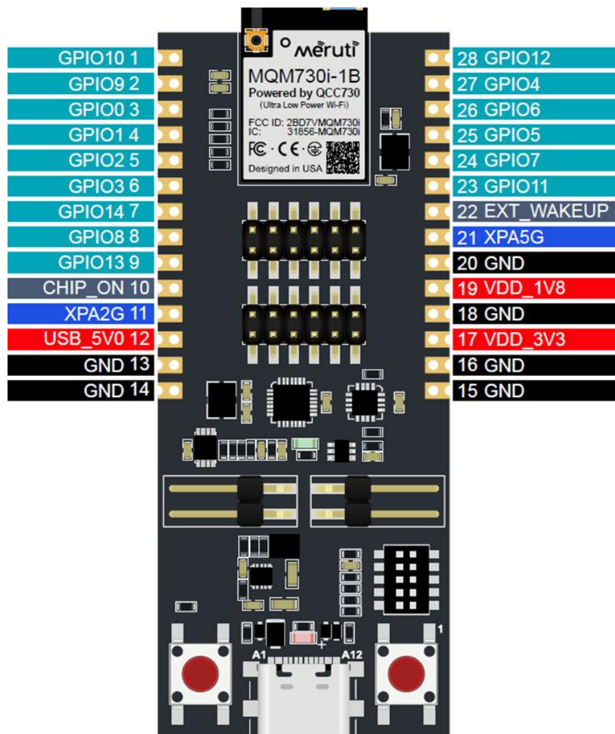
Figure 5: QCC730 Module Development Kit Pin Map
