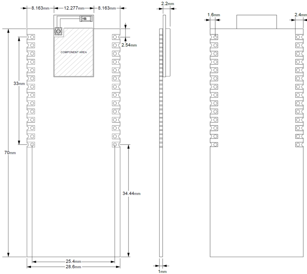
Figure 8: QCC730 Module Development Kit Dimension
