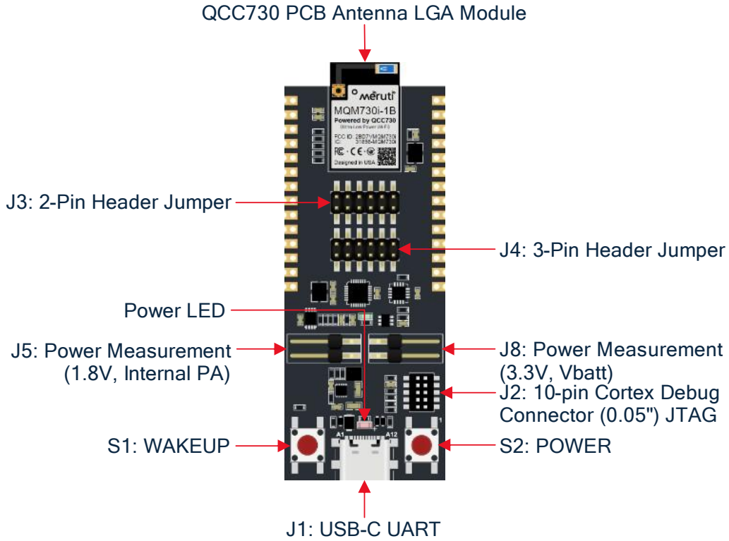
Figure 6: QCC730 Module Development Kit Component Layout
