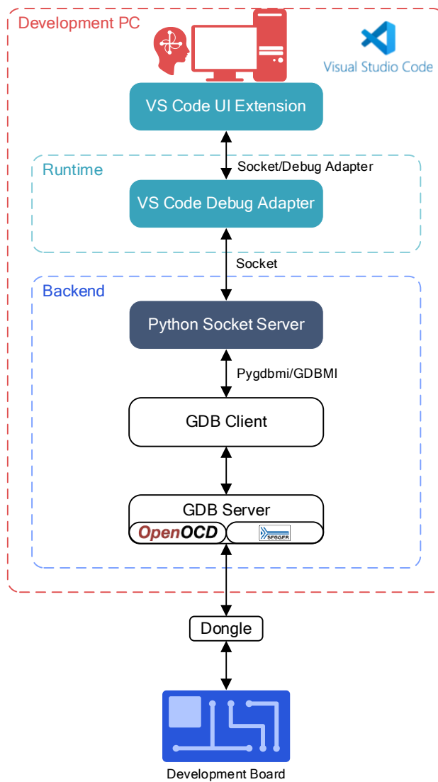
Figure 12: QCC730 Module Development Kit VS Code IDE Architecture
