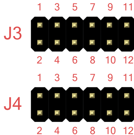
Figure 7: QCC730 Module Development Kit Jumper Setting
