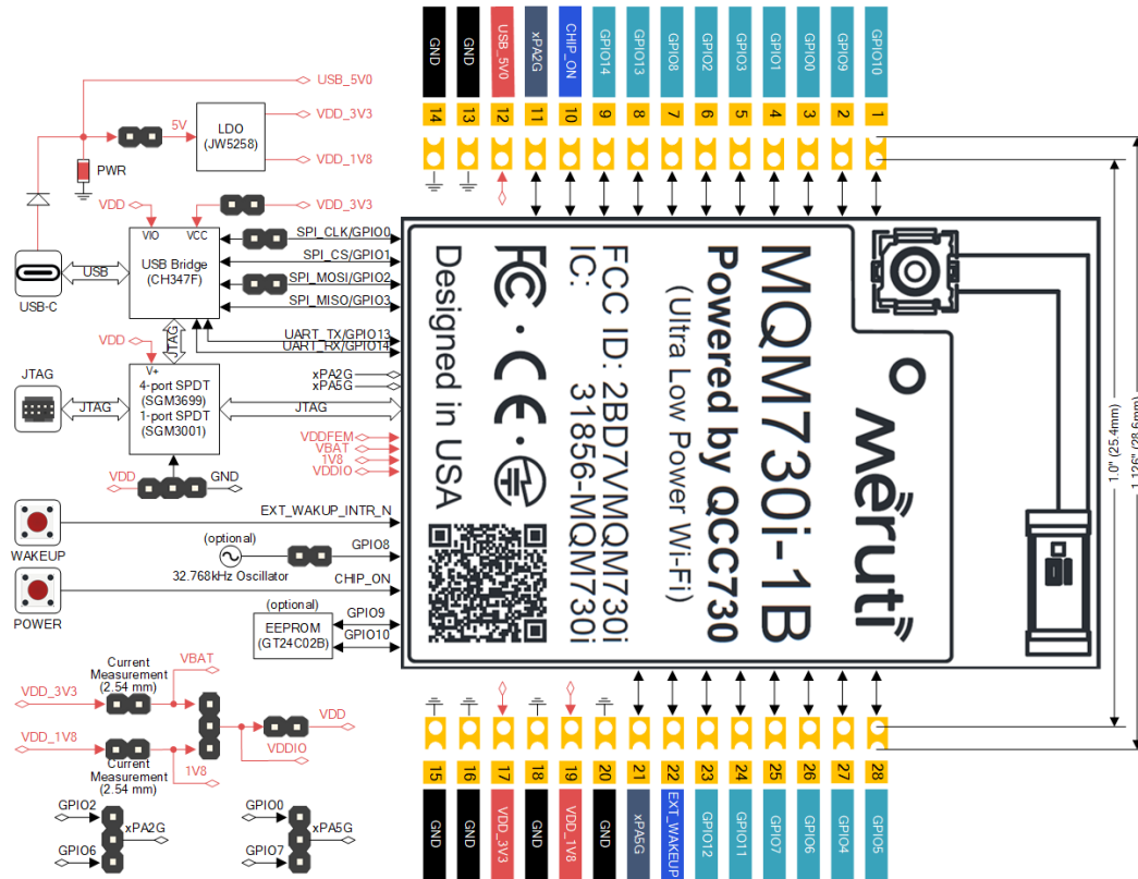
Figure 4: QCC730 Module Development Kit Block Diagram
