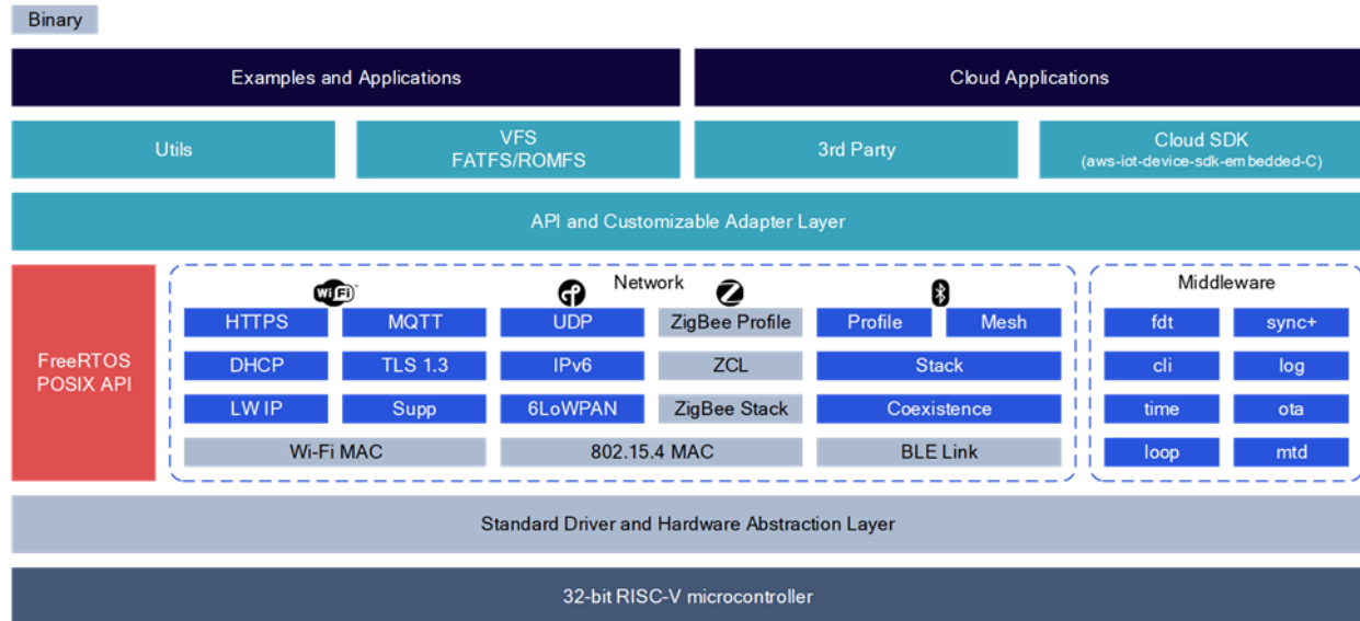
Figure 10: QCC744 Module Development Kit SDK Software Architecture
