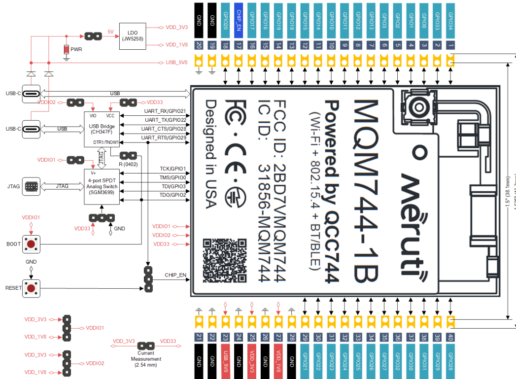
Figure 4: QCC744 Module Development Kit Block Diagram
