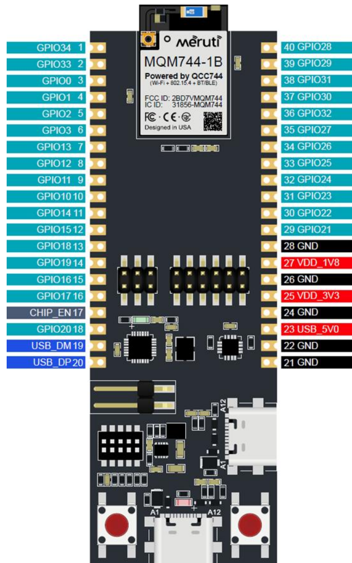
Figure 5: QCC744 Module Development Kit Pin Map
