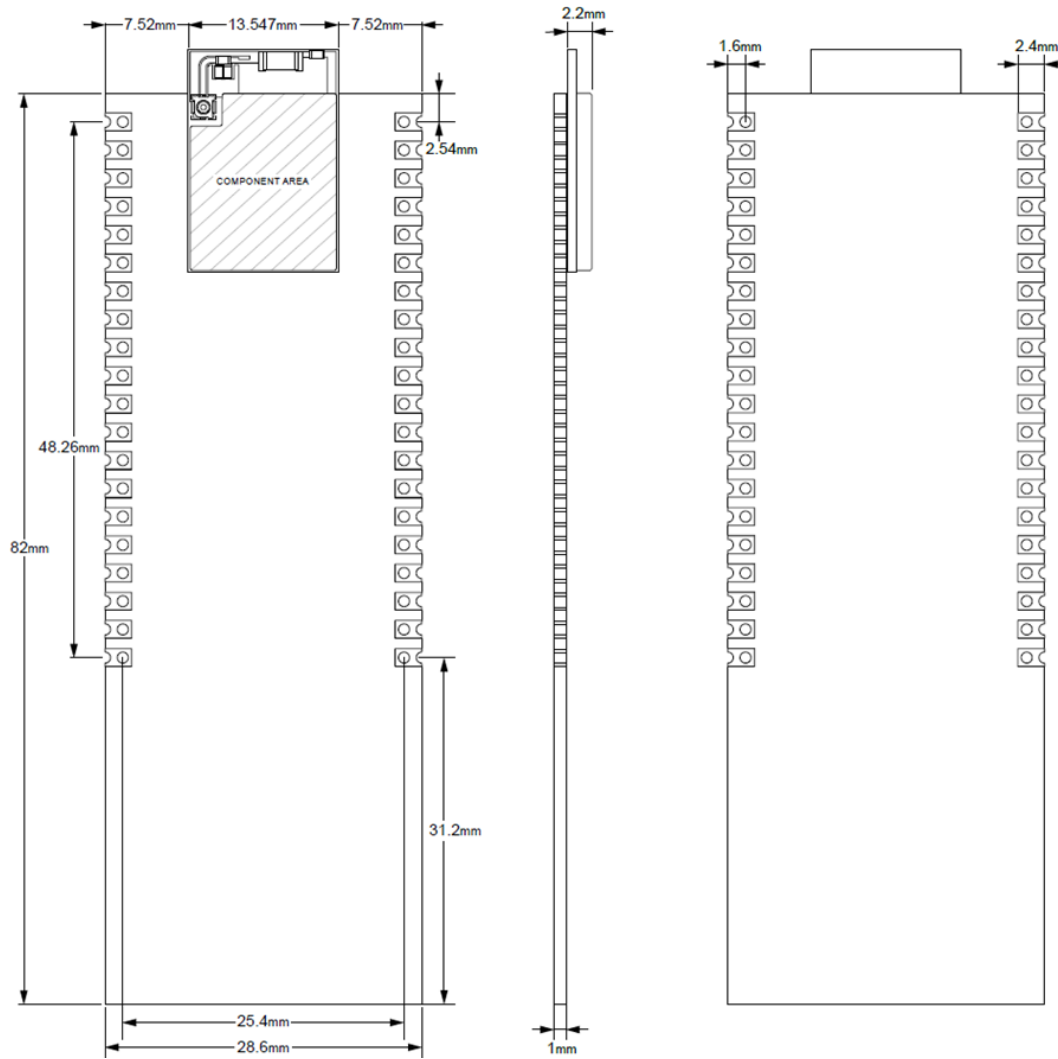
Figure 8: QCC744 Module Development Kit Dimension
