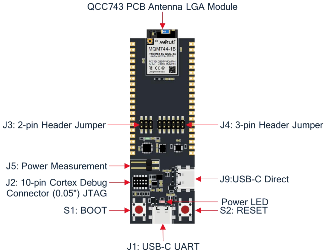
Figure 6: QCC744 Module Development Kit Component Layout
