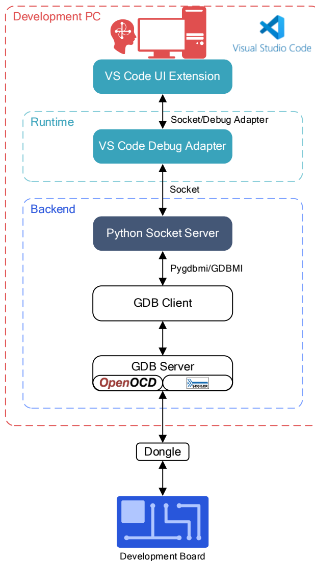
Figure 12: QCC744 Module Development Kit VS Code IDE Architecture
